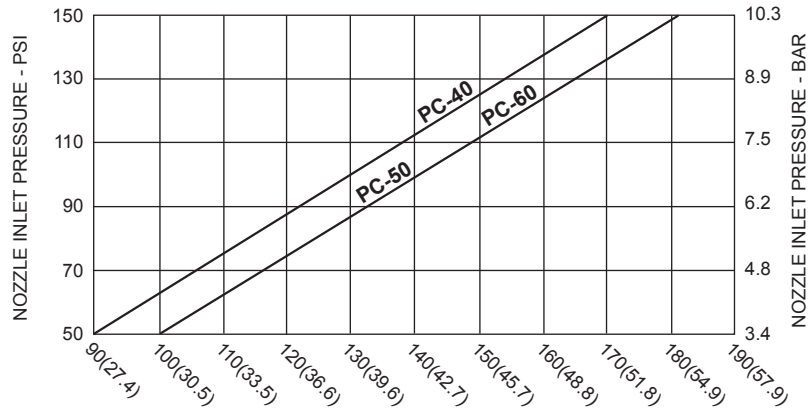
STRAIGHT STREAM RANGE IN FEET (METERS) STILL AIR (Range is with nozzle elevated 22.5° and nozzle inlet 3 to 6 feet (1 to 2 meters) above ground level)
