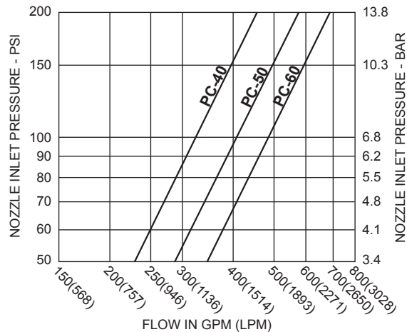
WATER OR FOAM SOLUTION NOZZLE DISCHARGE CHARACTERISTICS
