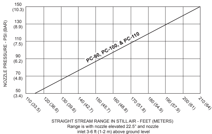
RANGE CHARACTERISTICS OF STRAIGHT STREAM NOZZLES
