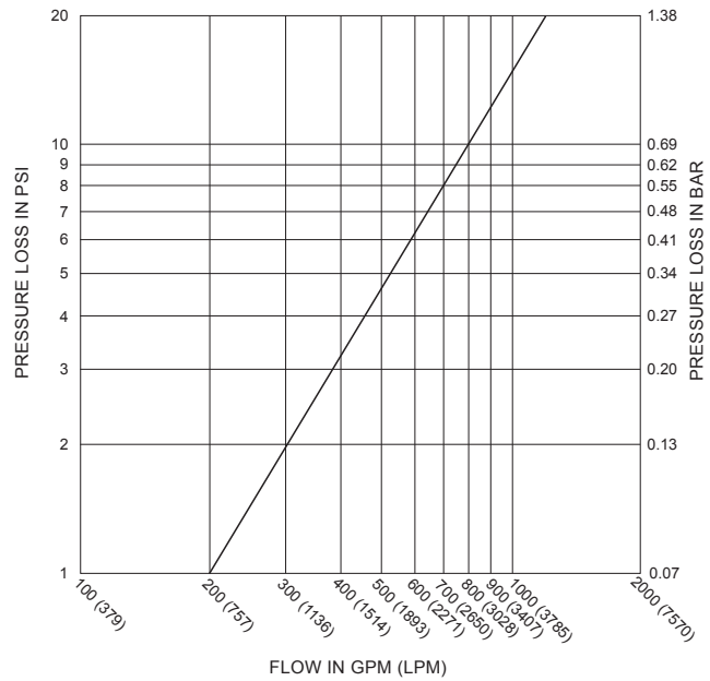
MODEL MMB-3 X 2-1/2 MONITOR PRESSURE LOSS VS FLOW
