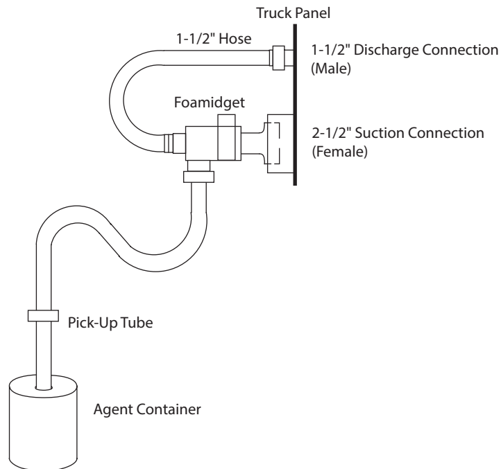
FoaMidget- Typical Set-Up
