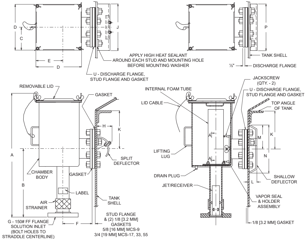
FOAM CHAMBER SECTION WITH SHALLOW DEFLECTOR
