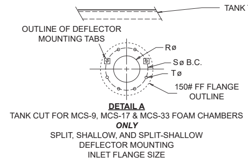
FOAM CHAMBER WITH SPLIT DEFLECTOR & STUD FLANGE
