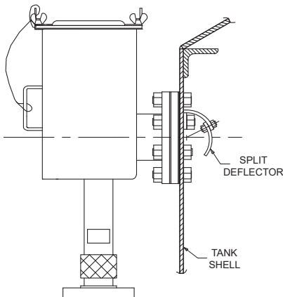
MCS CHAMBER with SPLIT DEFLECTOR ASSEMBLED
