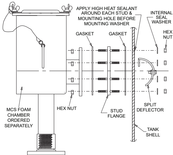
FOAM CHAMBER MOUNTING TO SPLIT DEFLECTOR KIT
