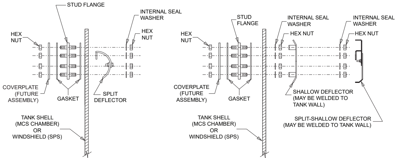
Split Deflector Kit
