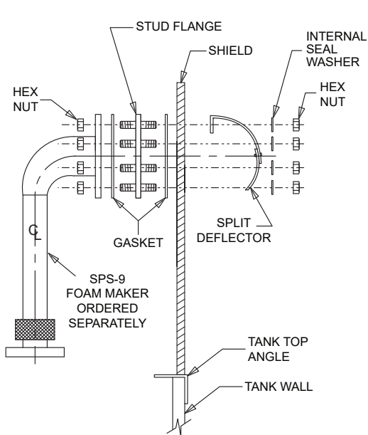
SPS-9 FOAM MAKER MOUNTING TO SPLIT DEFLECTOR KIT COMPONENTS on CUSTOMER SUPPLIED WINDSHIELD on OPEN TOP FLOATING ROOF TANK
