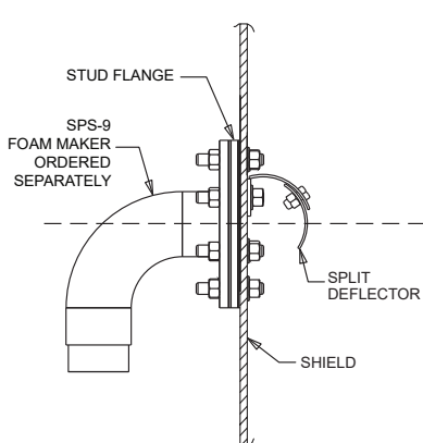
SPS-9FR FOAM DISCHARGE ASS'Y with SPLIT DEFLECTOR ASSEMBLED
