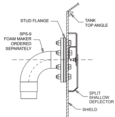
SPS-9FR FOAM DISCHARGE ASS'Y with SPLIT-SHALLOW DEFLECTOR ASSEMBLED
