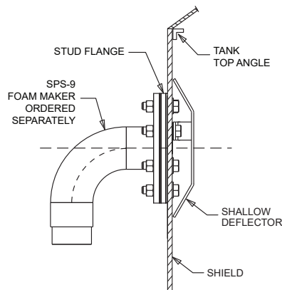
SPS-9FR FOAM DISCHARGE ASS'Y with SHALLOW DEFLECTOR ASSEMBLED
