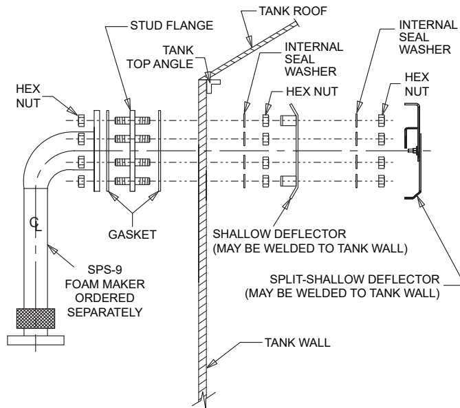
SPS-9 FOAM MAKER MOUNTING TO SHALLOW & SPLIT-SHALLOW DEFLECTOR KIT on INTERNAL FLOATING ROOF for SEAL PROTECTION ONLY
