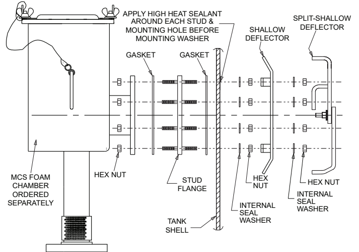
FOAM CHAMBER MOUNTING TO SHALLOW & SPLIT-SHALLOW DEFLECTOR KIT
