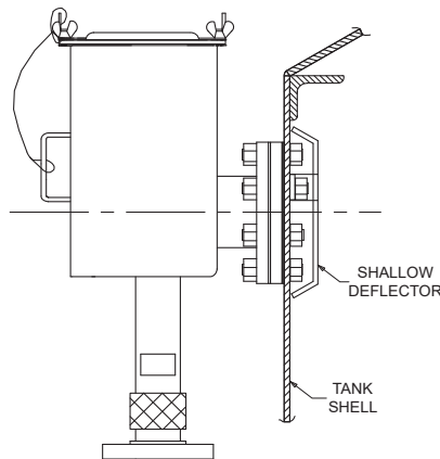
MCS CHAMBER with SHALLOW DEFLECTOR ASSEMBLED
