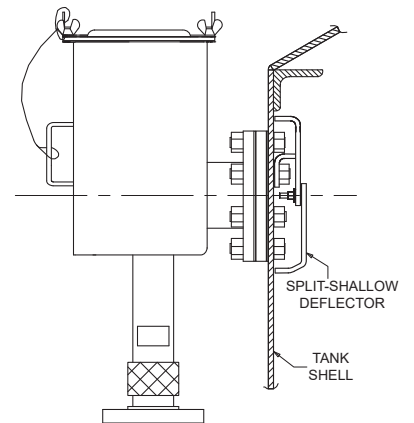
MCS CHAMBER with SPLIT-SHALLOW DEFLECTOR ASSEMBLED
