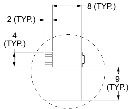
VIEW A BELT LOOP DETAIL (TYP. 8 PLACES) 2 PER SIDE
